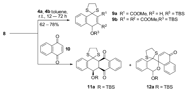
Scheme 4. Reaction of silyl ether 8 with alkynes 4 or 1,4-naphthoquinone 10 .
