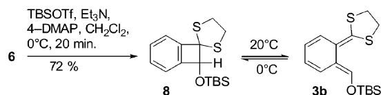
Scheme 3. Stabilization of benzocyclobutenol 6 as the silyl ether 8 and its electrocyclic ring-opening.
