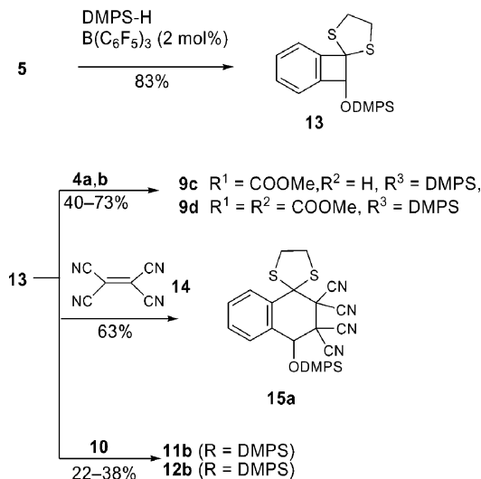
Scheme 5. Reaction of silyl ether 13 with alkynes 4 , 1,4-naphthoquinone ( 10 ), or tetracyanoethene ( 14 ).
