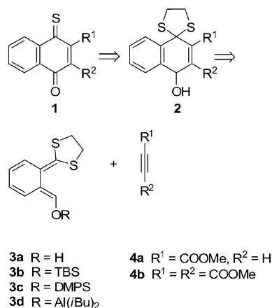
Scheme 1. A potential route to thionaphthoquinones.
