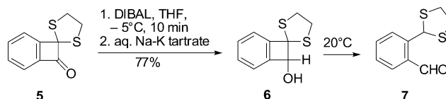
Scheme 2. Synthesis and rearrangement of benzocyclobutenol 6 .
