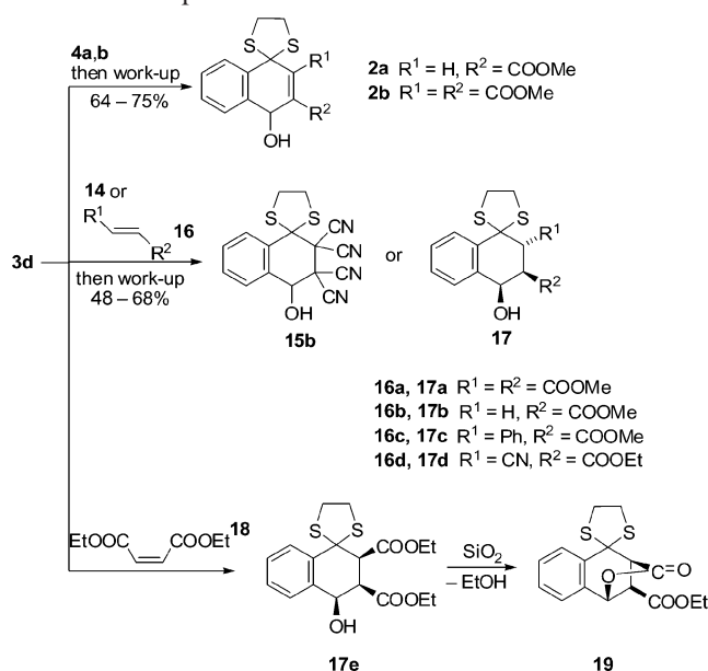
Scheme 6. Reaction of the aluminium salt 3d with dienophiles (only one enantiomer is shown; products after work-up).
